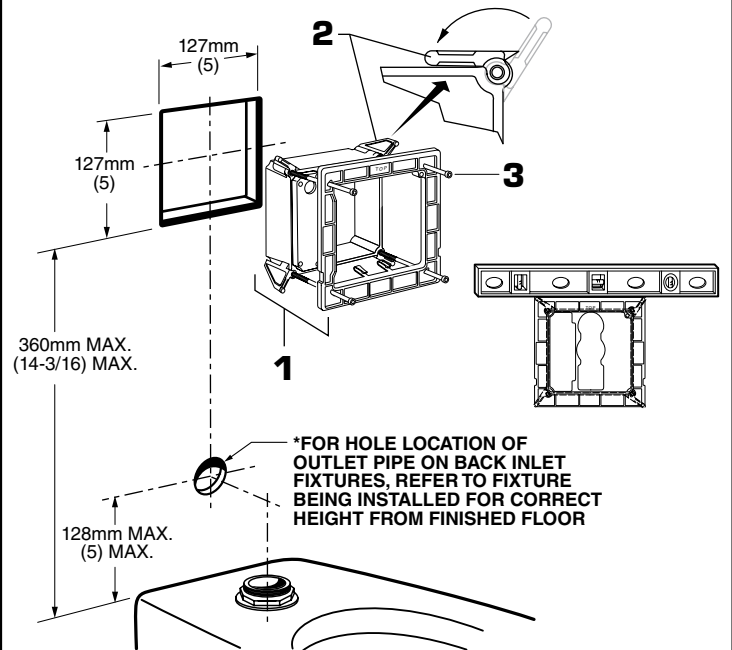
Fig.3 (TOP SPUD FIXTURE ILLUSTRATED)
